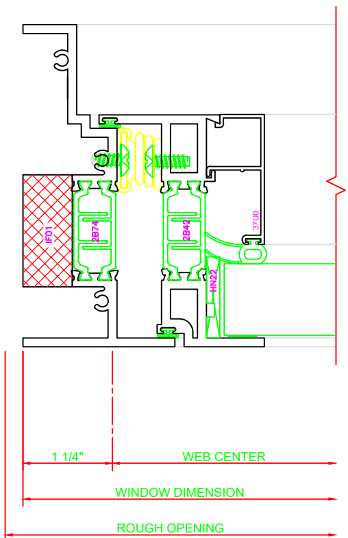
410 JAMB SERIES: 450X PROJECT IN 4-BAR ARMS
