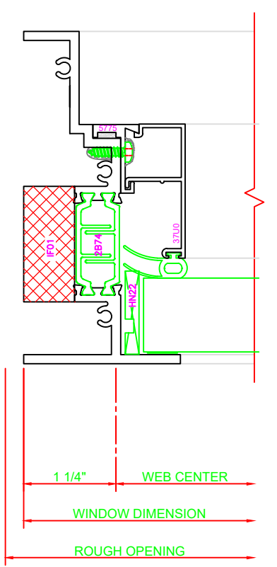
402 JAMB SERIES: 450X FIXED
