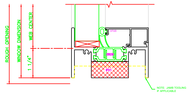
200 SILL 325 FIXED
