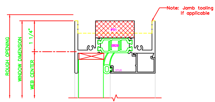
100 HEAD 325 FIXED
