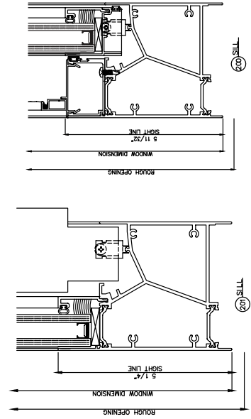
6551 XO Inside Glazed
